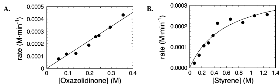
Figure 3. Kinetic data for the anti-Markovnikov oxidative amination of styrene with oxazolidinone (HNRZ) catalyzed by (\text{CH}_3\text{CN})_2\text{PdCl}_2 ( 1 ). Reaction conditions: (A) [\text{HNRZ}] = 0.055\text{--}0.355 \text{ M} , [\text{styrene}] = 1.26 \text{ M} , [\text{I}] = [\text{CuCl}_2] = 0.011 \text{ M} , p(\text{O}_2) = 1 \text{ atm} , DME, 60^\circ\text{C} ; (B) [\text{HNRZ}] = 0.23 \text{ M} , [\text{styrene}] = 0.079\text{--}1.27 \text{ M} , [\text{I}] = [\text{CuCl}_2] = 0.011 \text{ M} , p(\text{O}_2) = 1 \text{ atm} , DME, 60^\circ\text{C} . The line in plot A reflects a linear least-squares fit of the data. The saturation curve in plot B is obtained from a nonlinear least-squares fit to a generic hyperbolic function ( y = c_1[\text{St}]/(c_2[\text{St}] + c_3) ), the specific form of which is described in the Results and Discussion (eq 6).
