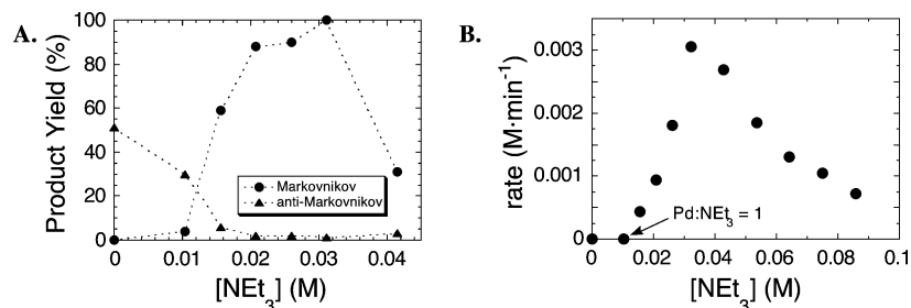
Figure 2. Effect of [\text{NEt}_3] on the product distribution (A) and the initial rate of Markovnikov product formation (B). Reaction conditions: (A) [\text{styrene}] = 1.26 \text{ M} , [\text{HNRZ}] = 0.21 \text{ M} , [(\text{CH}_3\text{CN})_2\text{PdCl}_2] = [\text{CuCl}_2] = 0.011 \text{ M} , [\text{NEt}_3] = 0\text{--}0.042 \text{ M} , p(\text{O}_2) = 1 \text{ atm} , DME, 60^\circ\text{C} , 24 h; (B) [\text{styrene}] = 1.30 \text{ M} , [\text{HNRZ}] = 0.25 \text{ M} , [(\text{CH}_3\text{CN})_2\text{PdCl}_2] = [\text{CuCl}_2] = 0.013 \text{ M} , [\text{NEt}_3] = 0\text{--}0.086 \text{ M} , p(\text{O}_2) = 1 \text{ atm} , DME, 60^\circ\text{C} .
